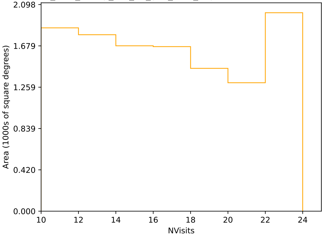
too_elab_heavy_r64_d3_griz_v3.4_10yrs Yr 3-4 r band: NVisits
