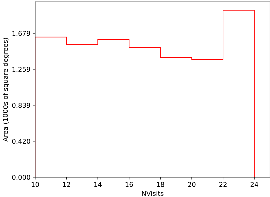
too_elab_heavy_r64_d3_griz_v3.4_10yrs Yr 3-4 i band: NVisits
