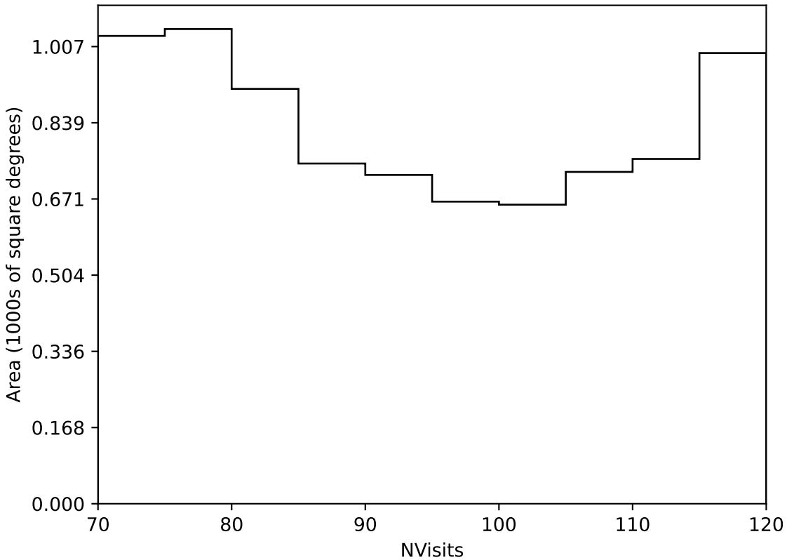
too_elab_heavy_r64_d3_griz_v3.4_10yrs Yr 3-4 all bands: NVisits
