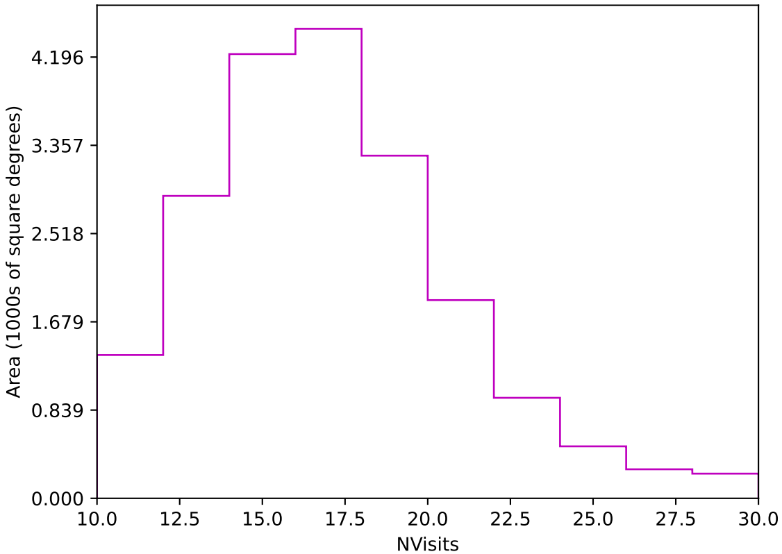
too_elab_heavy_r64_d3_griz_v3.4_10yrs Yr 1 z band: NVisits
