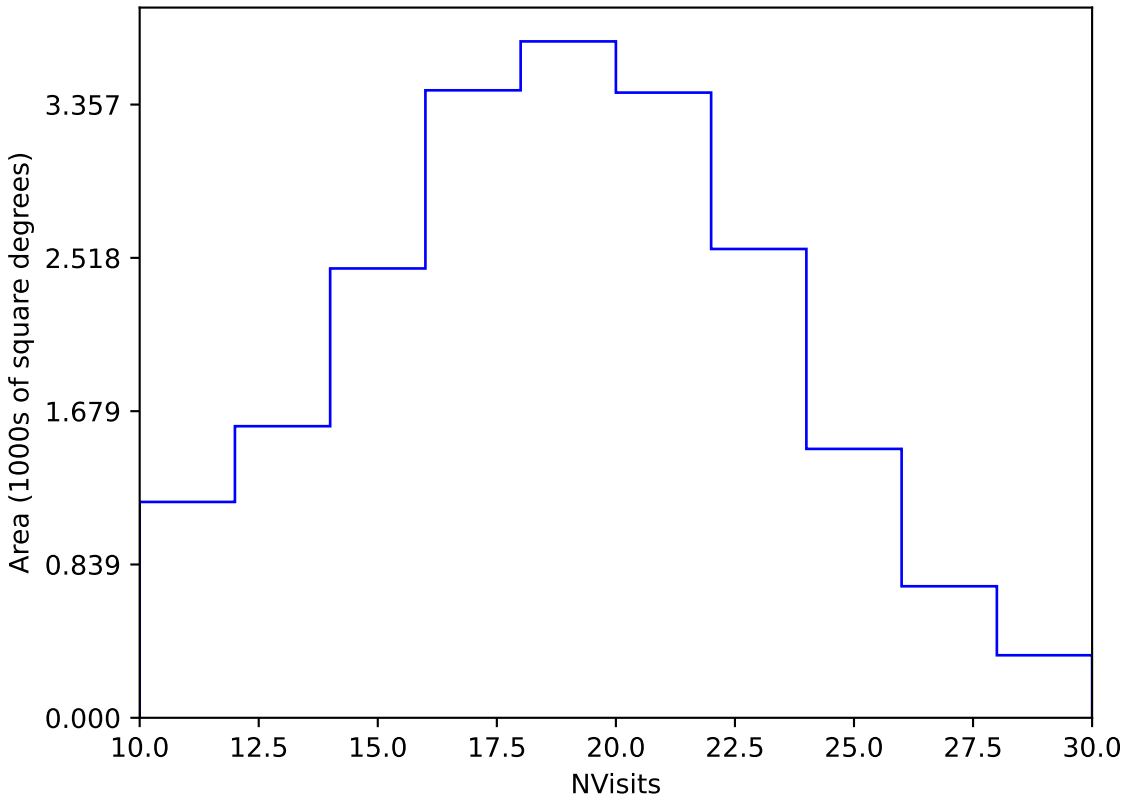
too_elab_heavy_r64_d3_griz_v3.4_10yrs Yr 1 y band: NVisits
