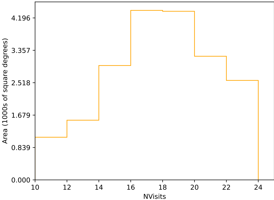
too_elab_heavy_r64_d3_griz_v3.4_10yrs Yr 1 r band: NVisits
