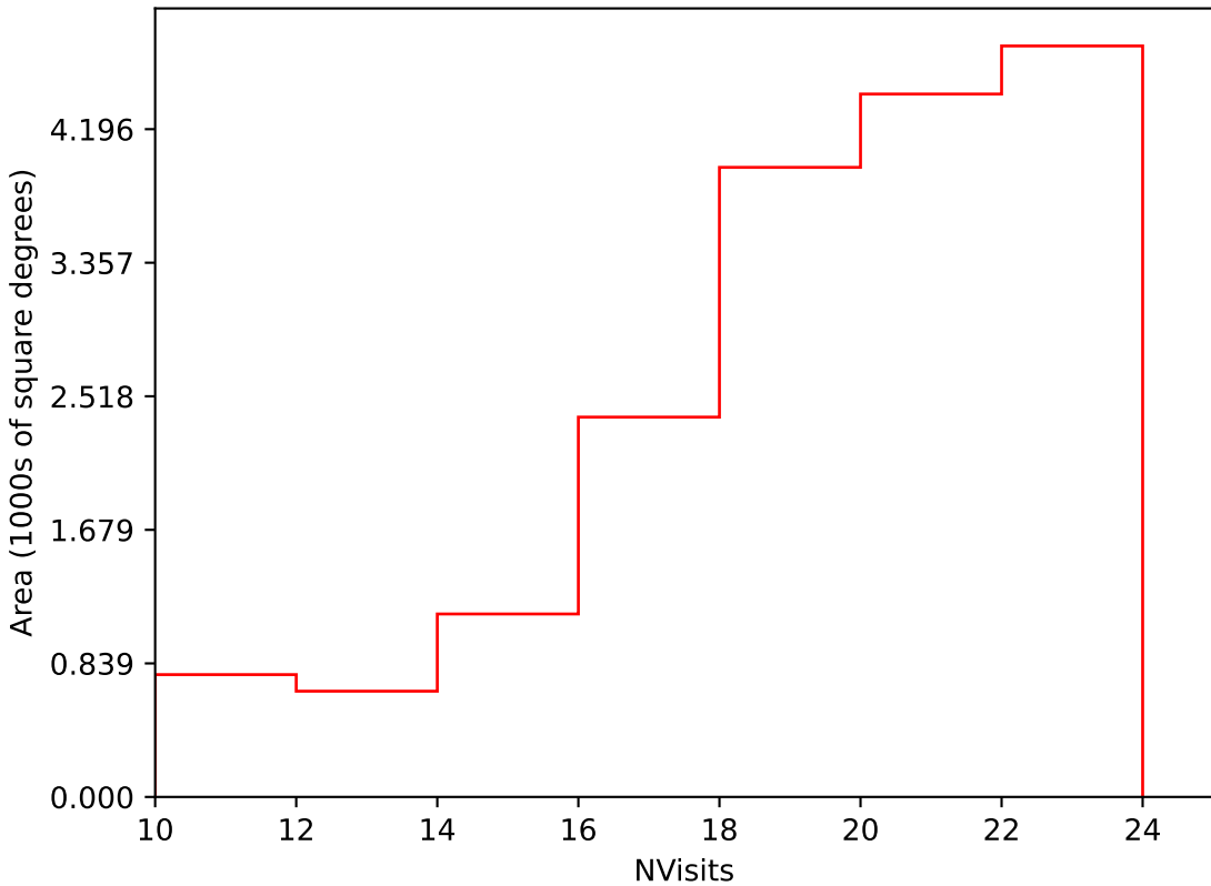
too_elab_heavy_r64_d3_griz_v3.4_10yrs Yr 1 i band: NVisits
