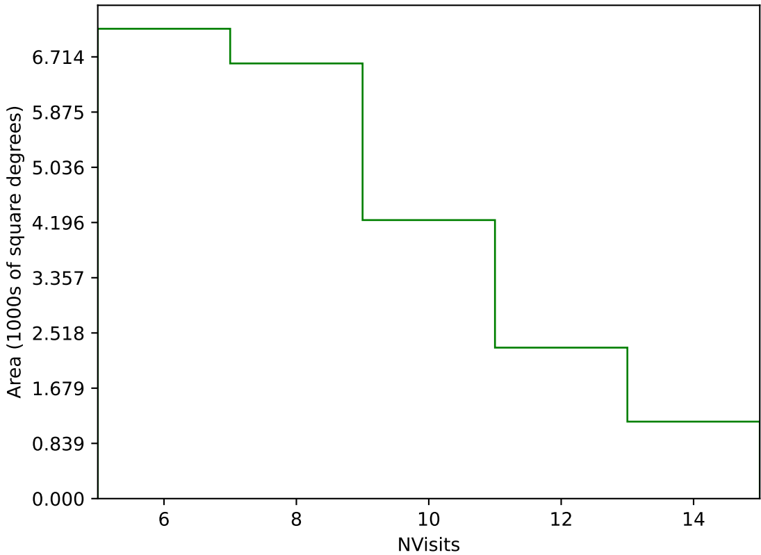
too_elab_heavy_r64_d3_griz_v3.4_10yrs Yr 1 g band: NVisits
