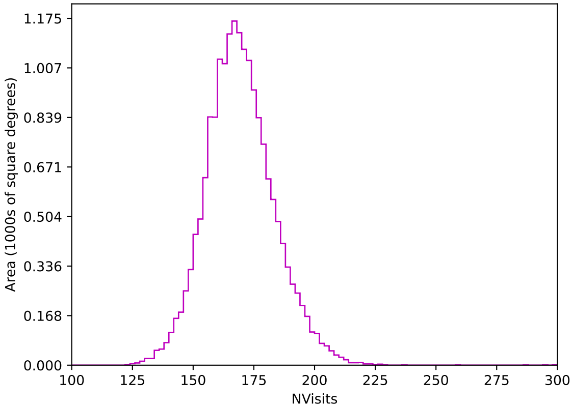
too_elab_heavy_r64_d3_griz_v3.4_10yrs WFD z band: NVisits
