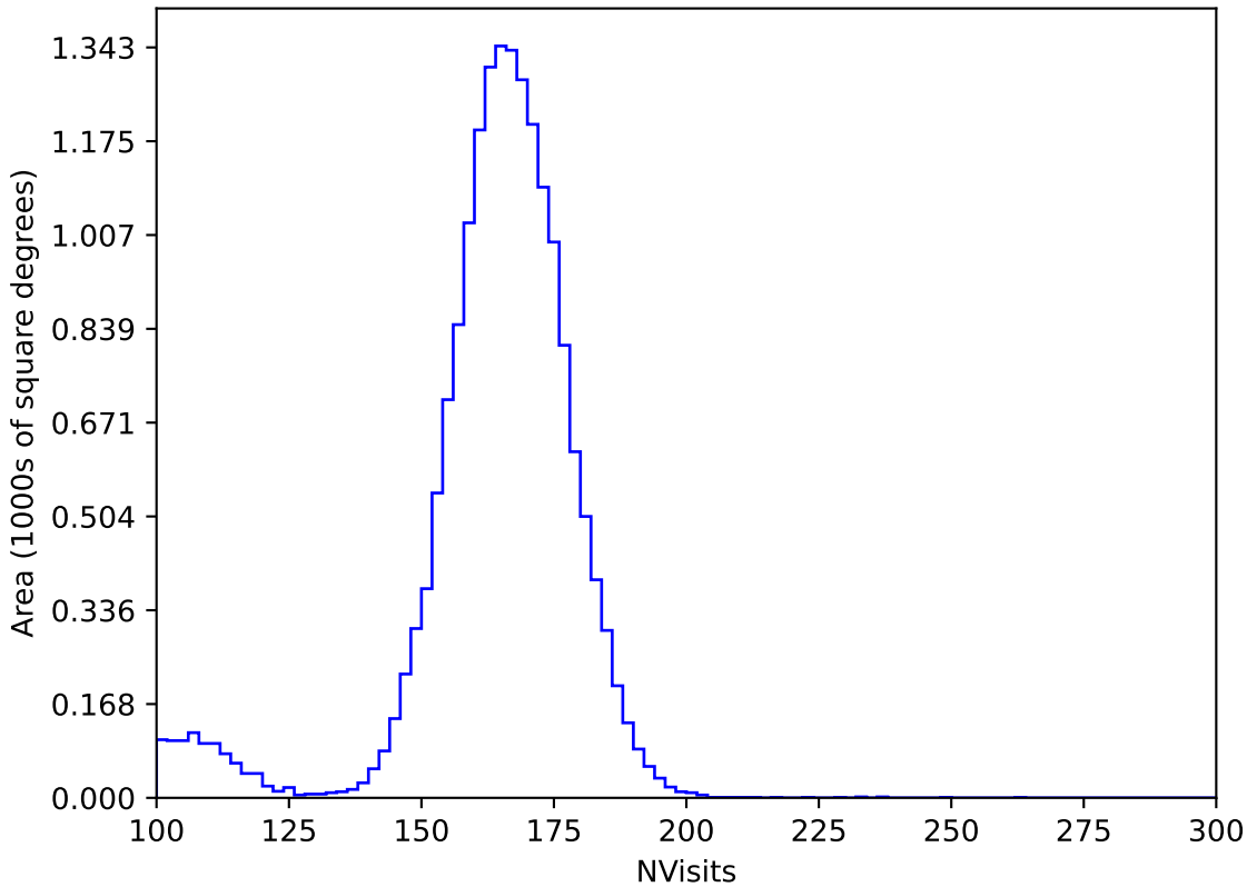
too_elab_heavy_r64_d3_griz_v3.4_10yrs WFD y band: NVisits
