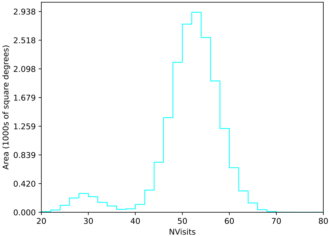
too_elab_heavy_r64_d3_griz_v3.4_10yrs WFD u band: NVisits
