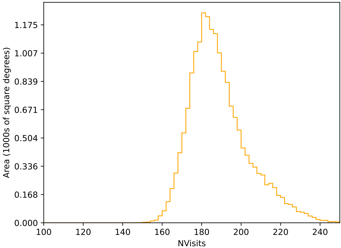
too_elab_heavy_r64_d3_griz_v3.4_10yrs WFD r band: NVisits
