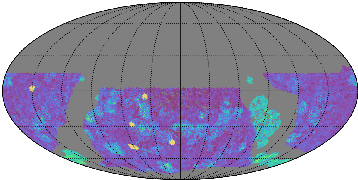
too_elab_heavy_r64_d3_griz_v3.4_10yrs WFD g band: NVisits
