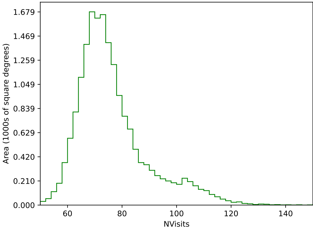
too_elab_heavy_r64_d3_griz_v3.4_10yrs WFD g band: NVisits
