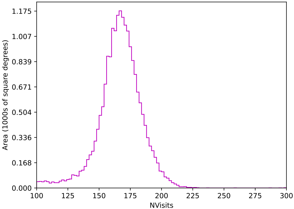
too_elab_heavy_r64_d3_griz_v3.4_10yrs All sky z band: NVisits
