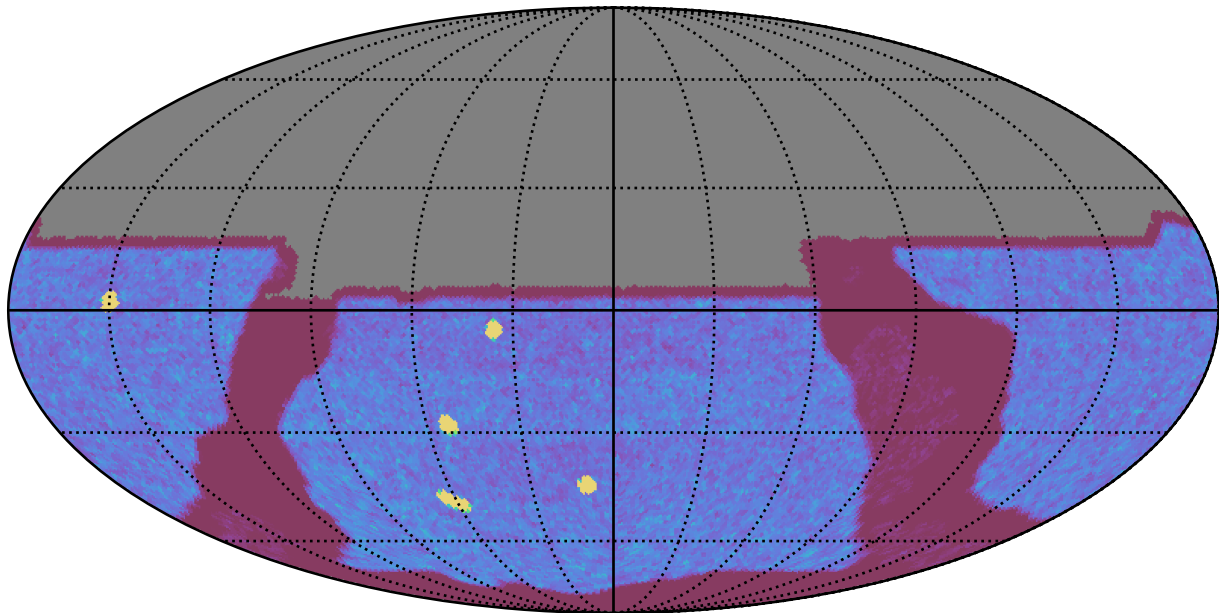
too_elab_heavy_r64_d3_griz_v3.4_10yrs All sky y band: NVisits
