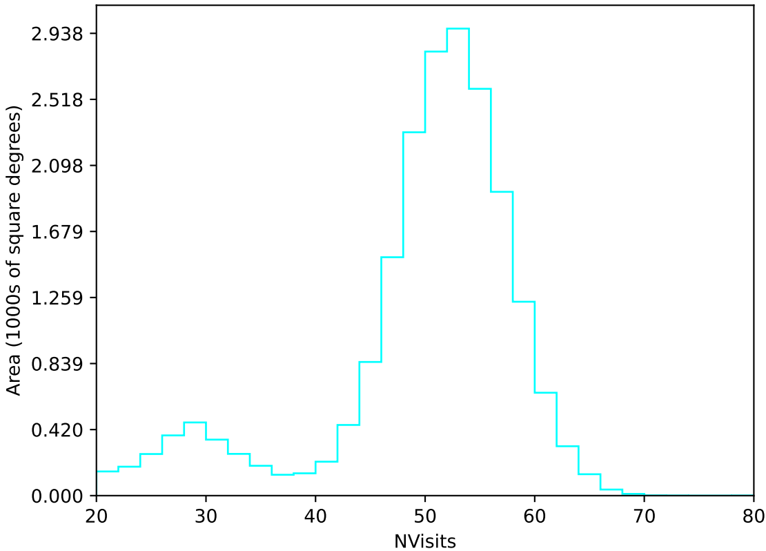
too_elab_heavy_r64_d3_griz_v3.4_10yrs All sky u band: NVisits
