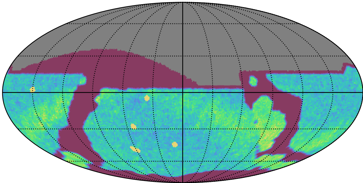
too_elab_heavy_r64_d3_griz_v3.4_10yrs All sky r band: NVisits
