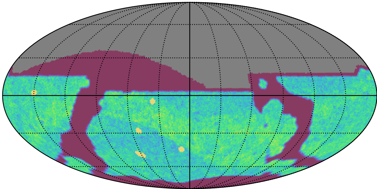
too_elab_heavy_r64_d3_griz_v3.4_10yrs All sky i band: NVisits
