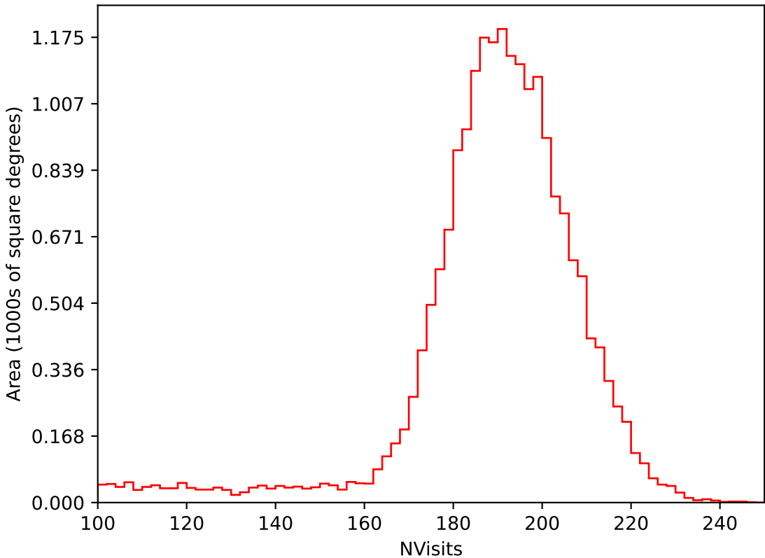
too_elab_heavy_r64_d3_griz_v3.4_10yrs All sky i band: NVisits
