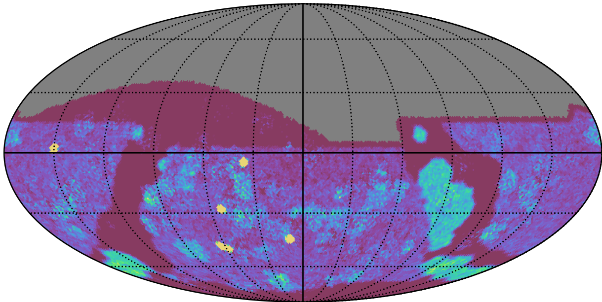
too_elab_heavy_r64_d3_griz_v3.4_10yrs All sky g band: NVisits
