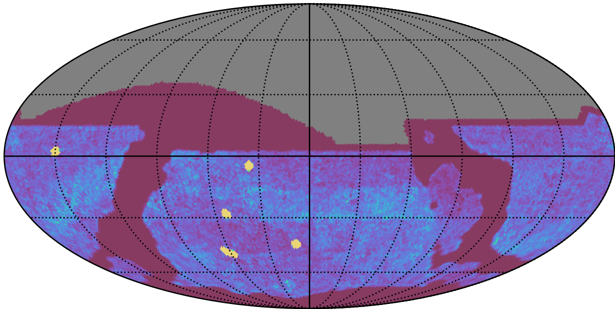
too_elab_heavy_r64_d3_griz_v3.4_10yrs All sky all bands: NVisits
