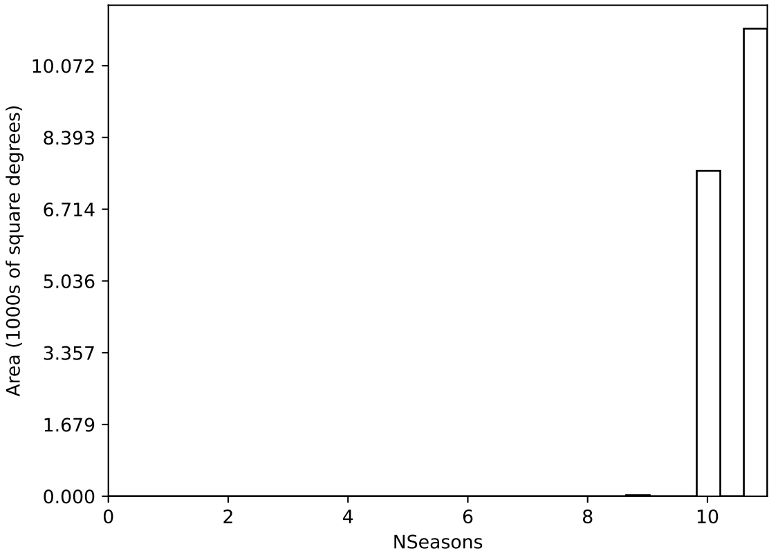
too_elab_heavy_r64_d3_griz_v3.4_10yrs WFD all bands: NSeasons
