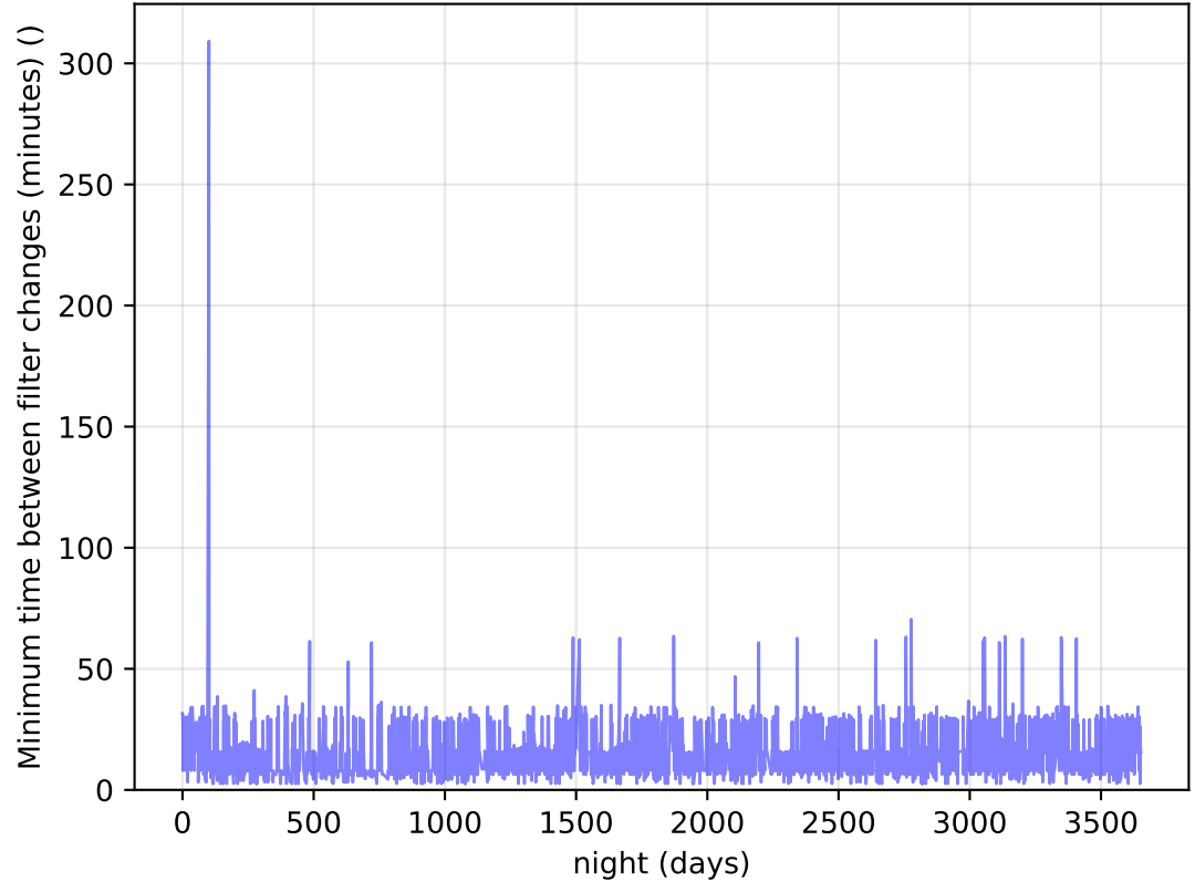
too_elab_heavy_r64_d3_griz_v3.4_10yrs Per Night: Minimum time between filter changes (minutes)
