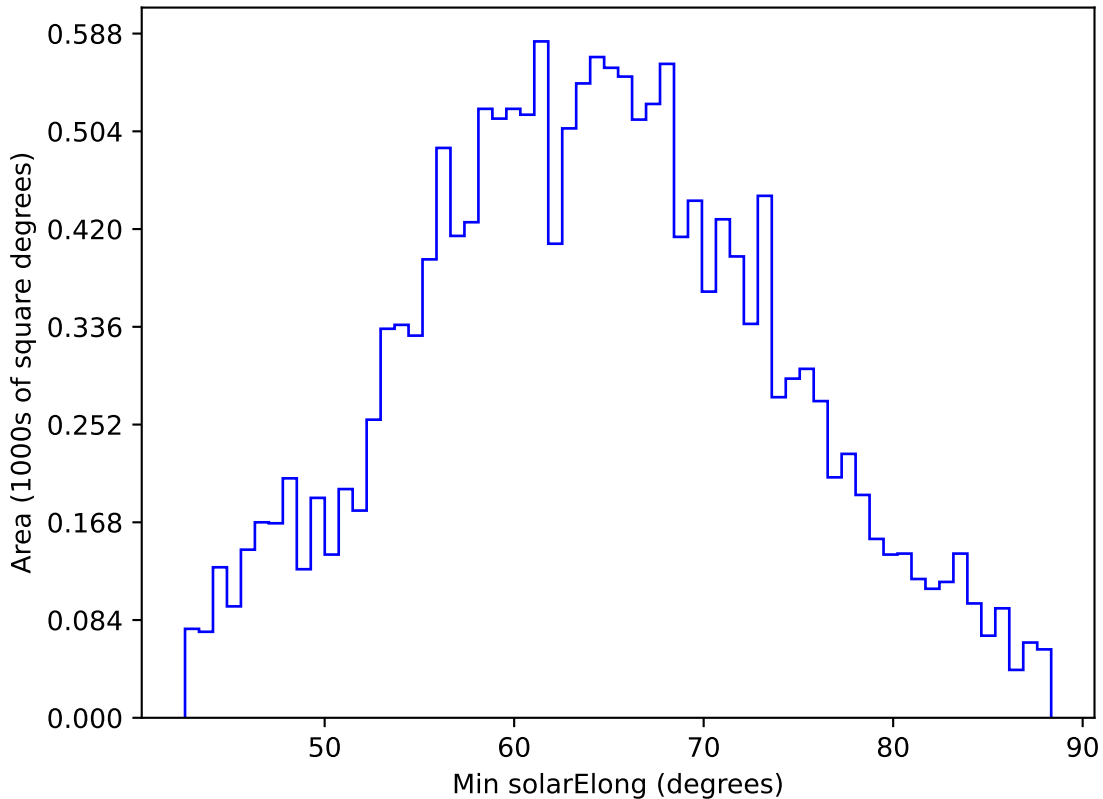
too_elab_heavy_r64_d3_griz_v3.4_10yrs WFD y band: Min solarElong
