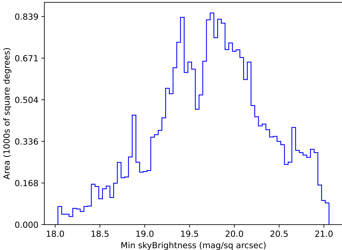
too_elab_heavy_r64_d3_griz_v3.4_10yrs Yr 1 r band: Min skyBrightness
