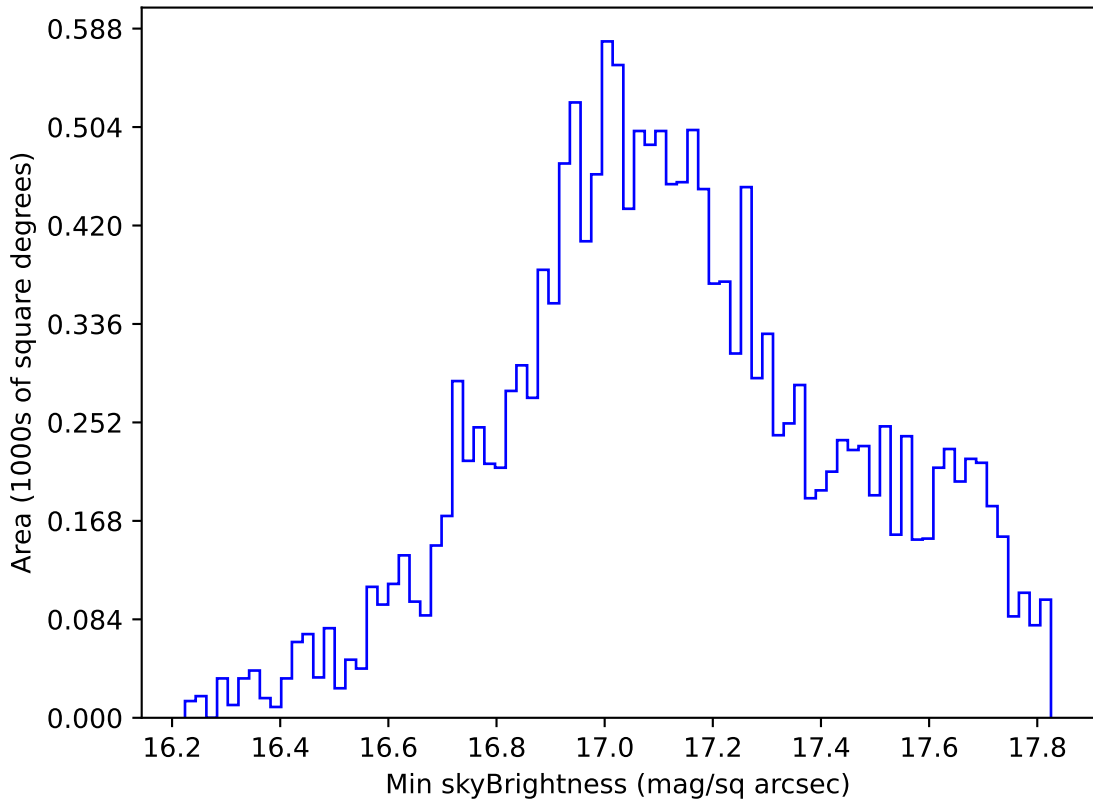
too_elab_heavy_r64_d3_griz_v3.4_10yrs WFD y band: Min skyBrightness
