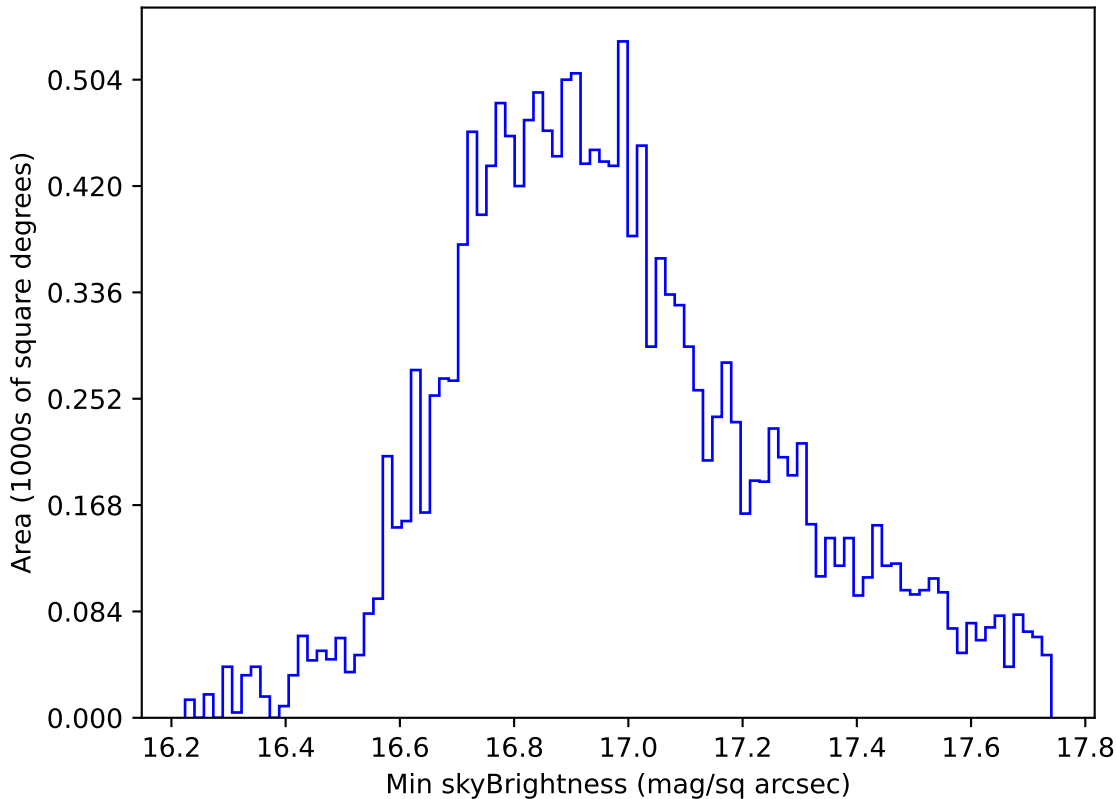
too_elab_heavy_r64_d3_griz_v3.4_10yrs WFD all bands: Min skyBrightness
