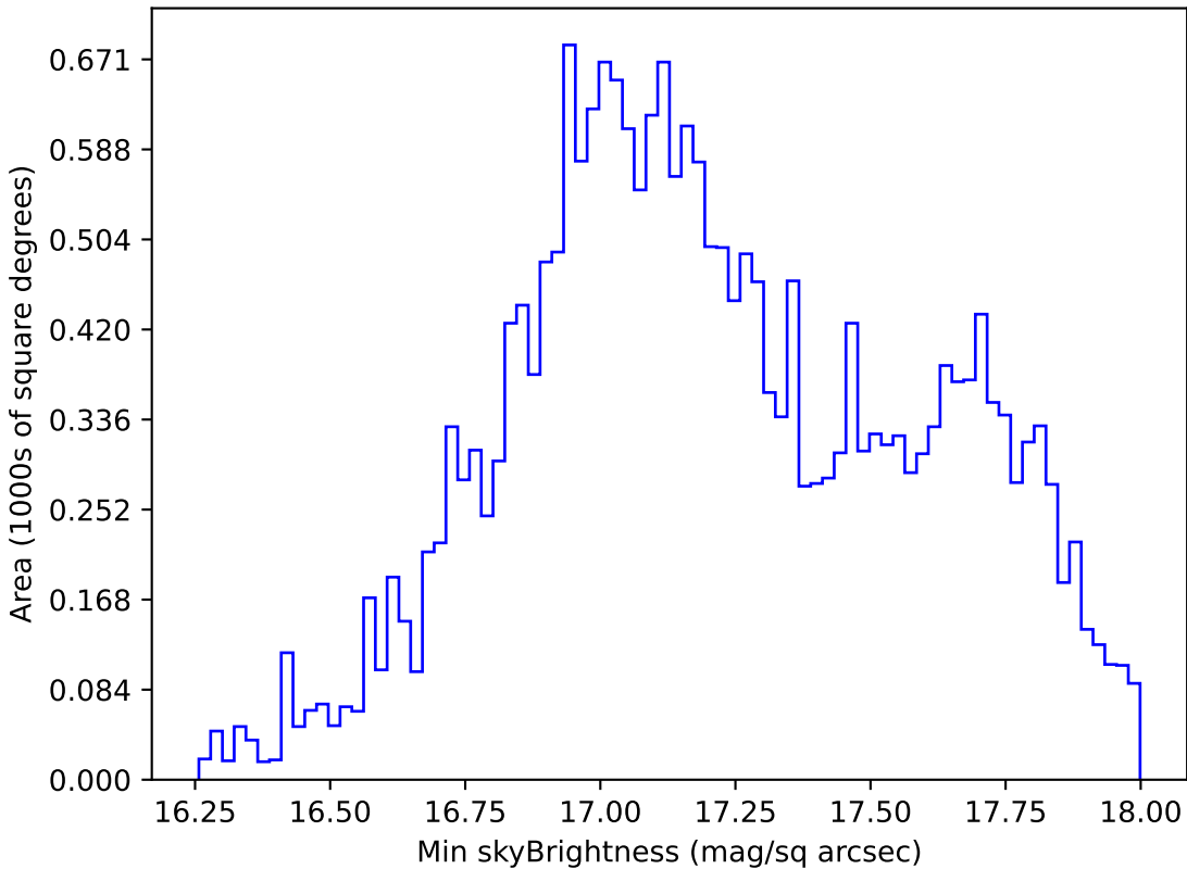
too_elab_heavy_r64_d3_griz_v3.4_10yrs All sky y band: Min skyBrightness
