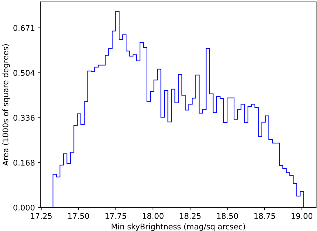
too_elab_heavy_r64_d3_griz_v3.4_10yrs All sky i band: Min skyBrightness
