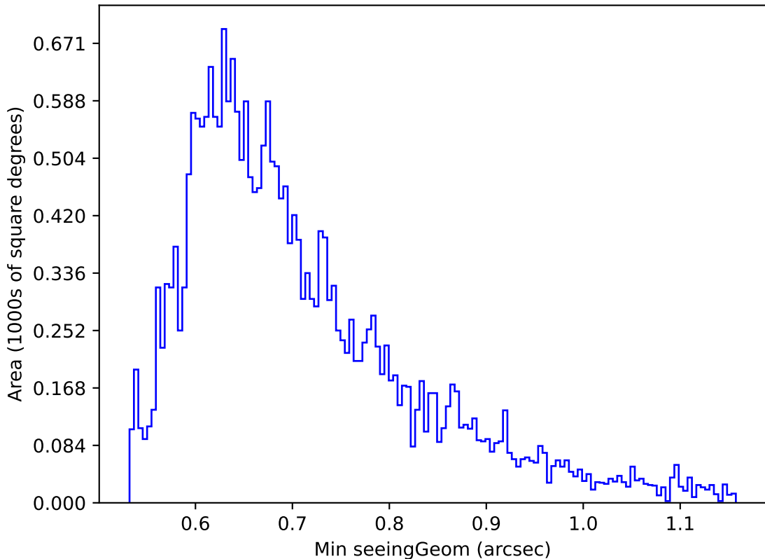
too_elab_heavy_r64_d3_griz_v3.4_10yrs Yr 1 g band: Min seeingGeom
