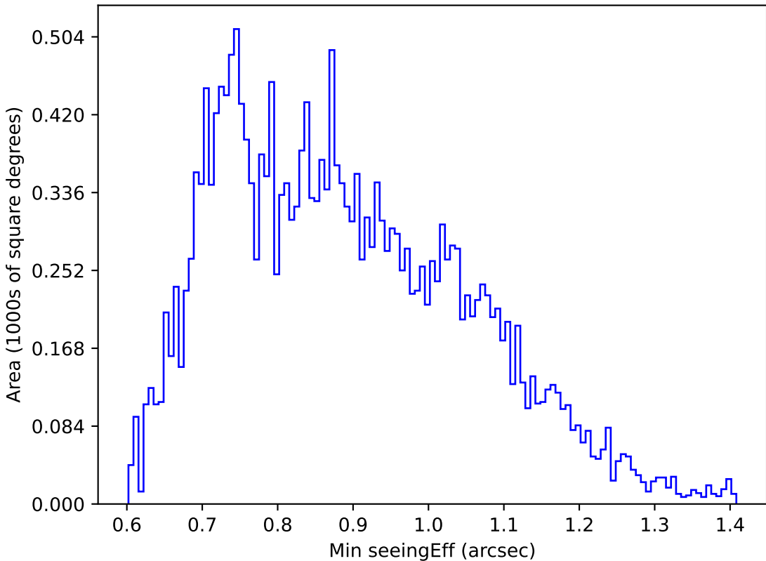
too_elab_heavy_r64_d3_griz_v3.4_10yrs Yr 1 u band: Min seeingEff
