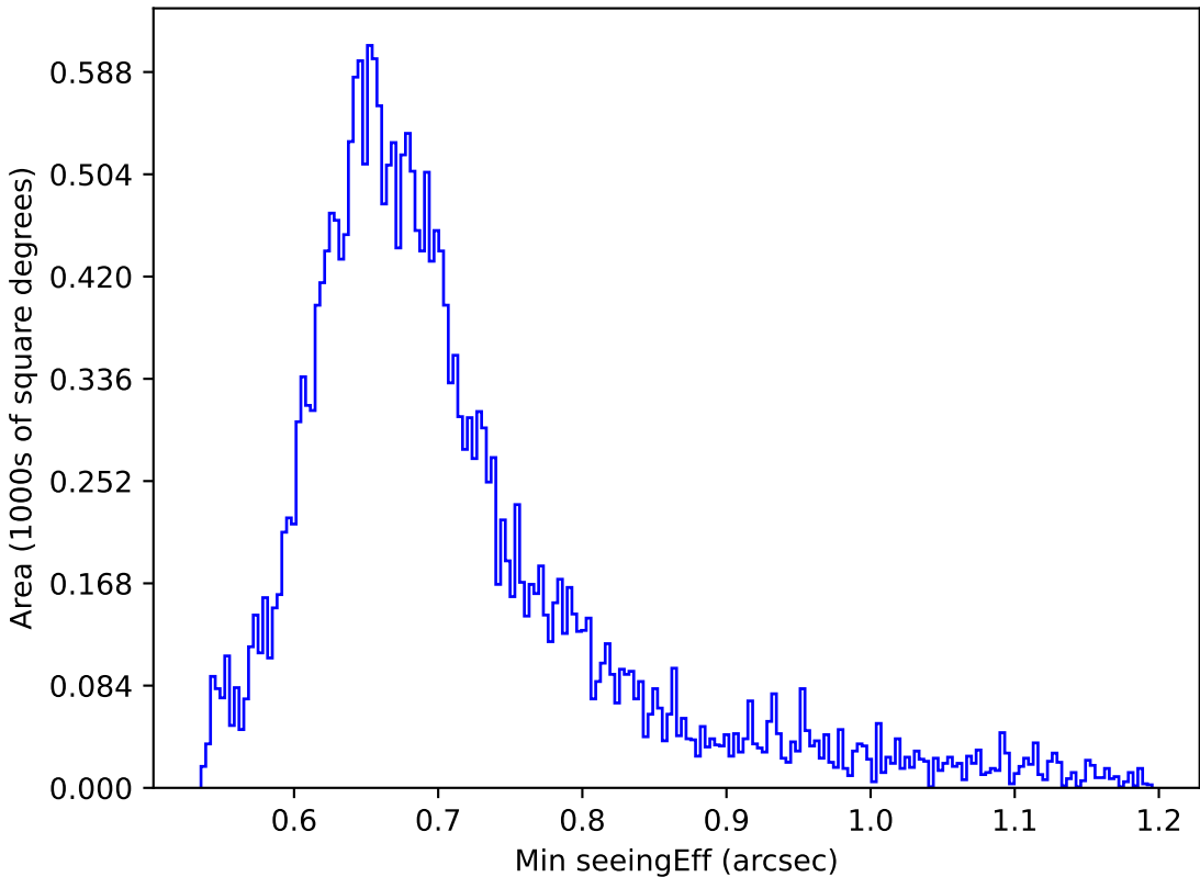
too_elab_heavy_r64_d3_griz_v3.4_10yrs Yr 1 i band: Min seeingEff
