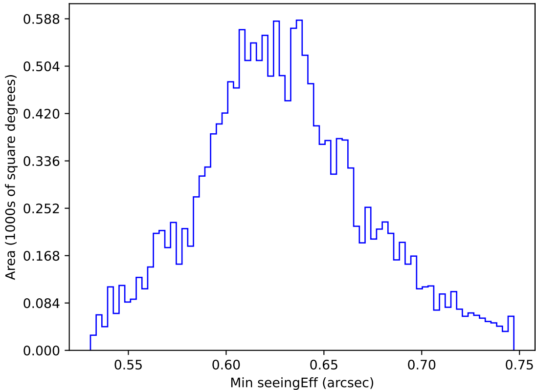
too_elab_heavy_r64_d3_griz_v3.4_10yrs WFD y band: Min seeingEff
