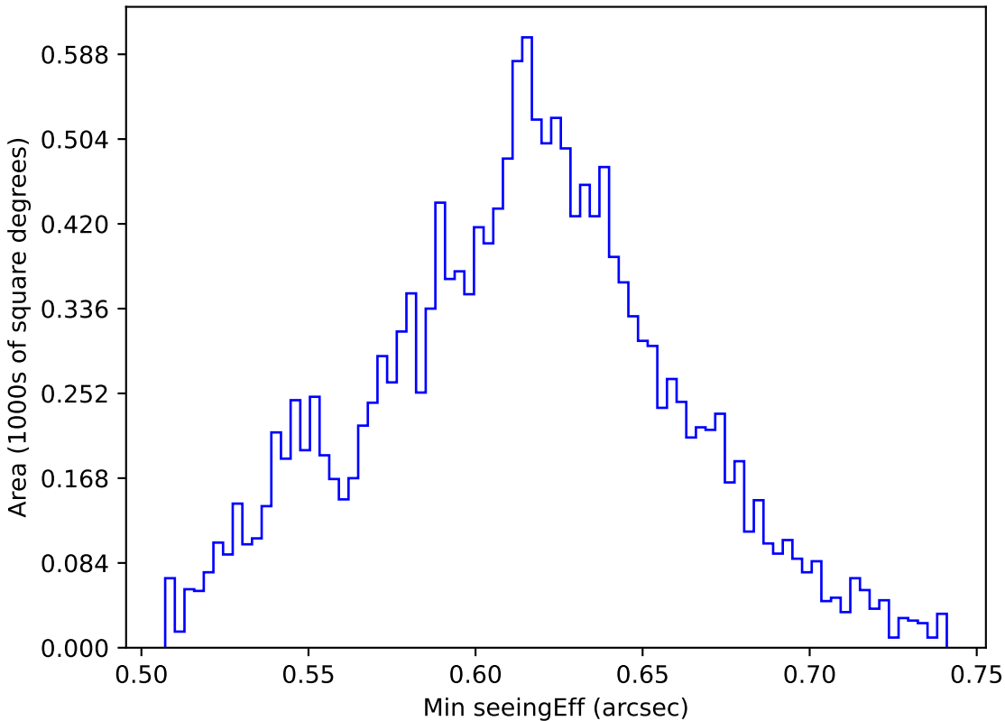
too_elab_heavy_r64_d3_griz_v3.4_10yrs WFD r band: Min seeingEff
