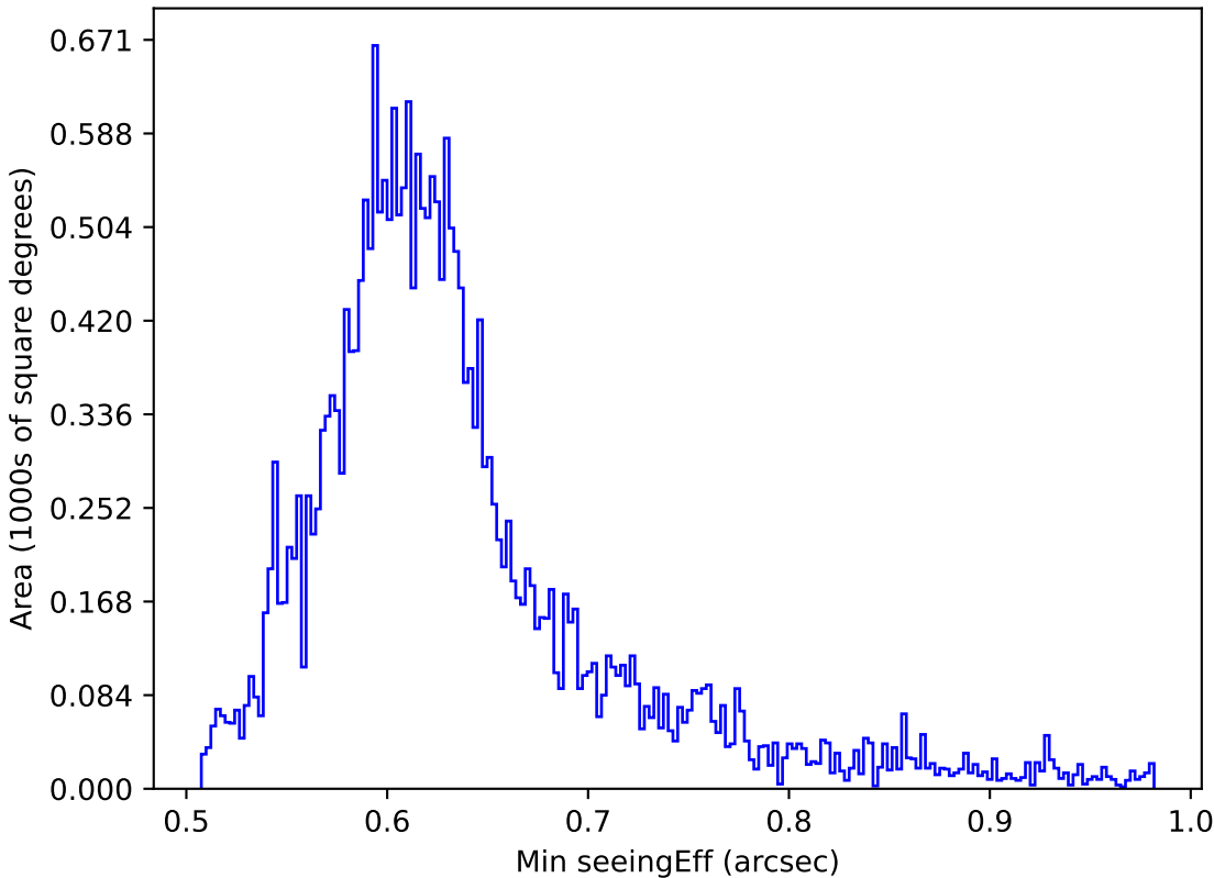
too_elab_heavy_r64_d3_griz_v3.4_10yrs All sky i band: Min seeingEff
