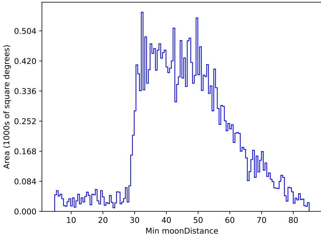
too_elab_heavy_r64_d3_griz_v3.4_10yrs All sky g band: Min moonDistance
