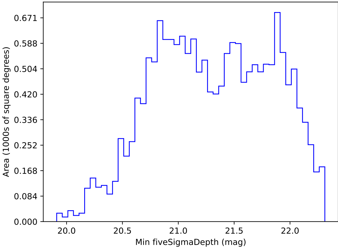
too_elab_heavy_r64_d3_griz_v3.4_10yrs WFD z band: Min fiveSigmaDepth
