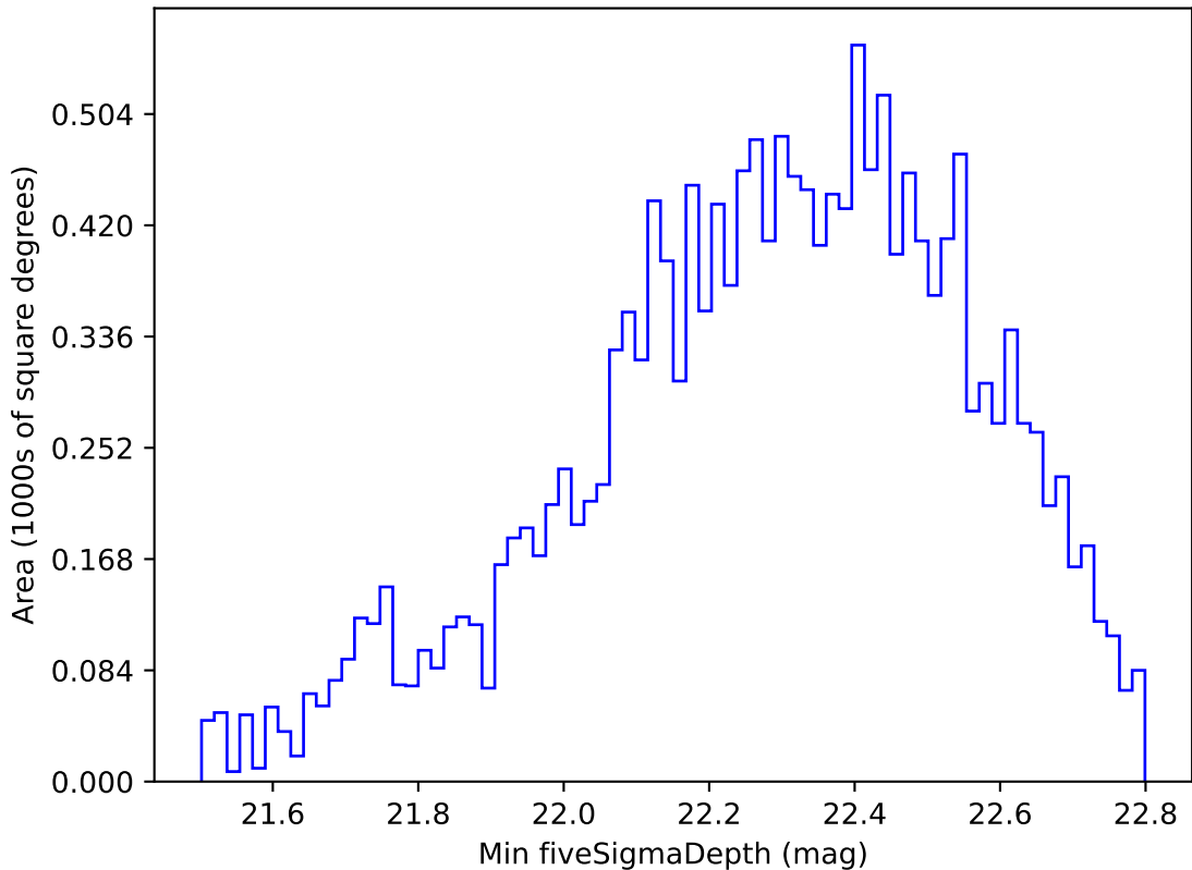
too_elab_heavy_r64_d3_griz_v3.4_10yrs WFD u band: Min fiveSigmaDepth
