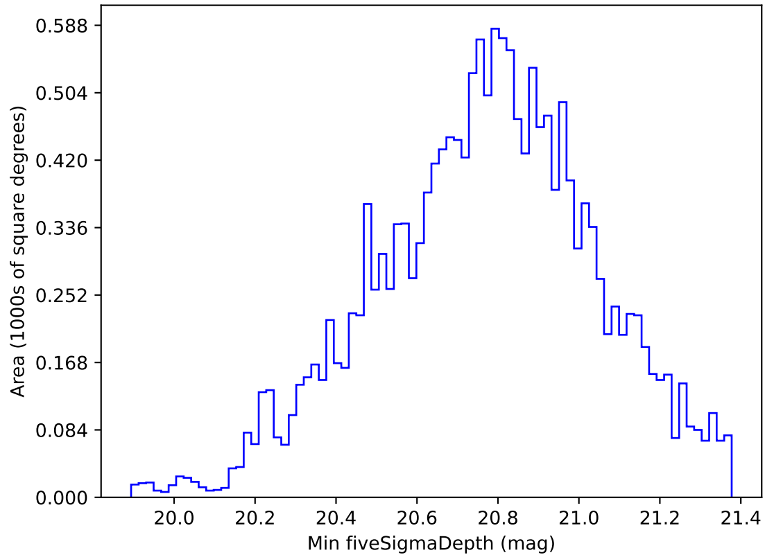
too_elab_heavy_r64_d3_griz_v3.4_10yrs WFD all bands: Min fiveSigmaDepth
