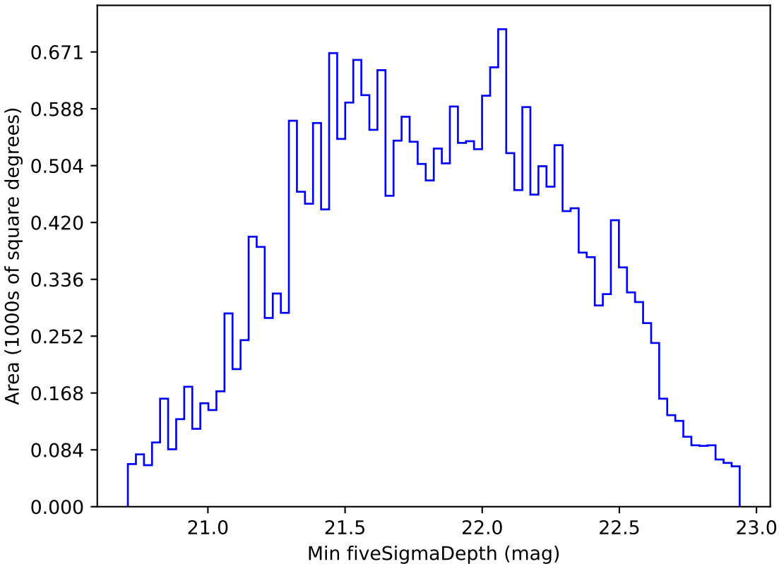
too_elab_heavy_r64_d3_griz_v3.4_10yrs All sky i band: Min fiveSigmaDepth
