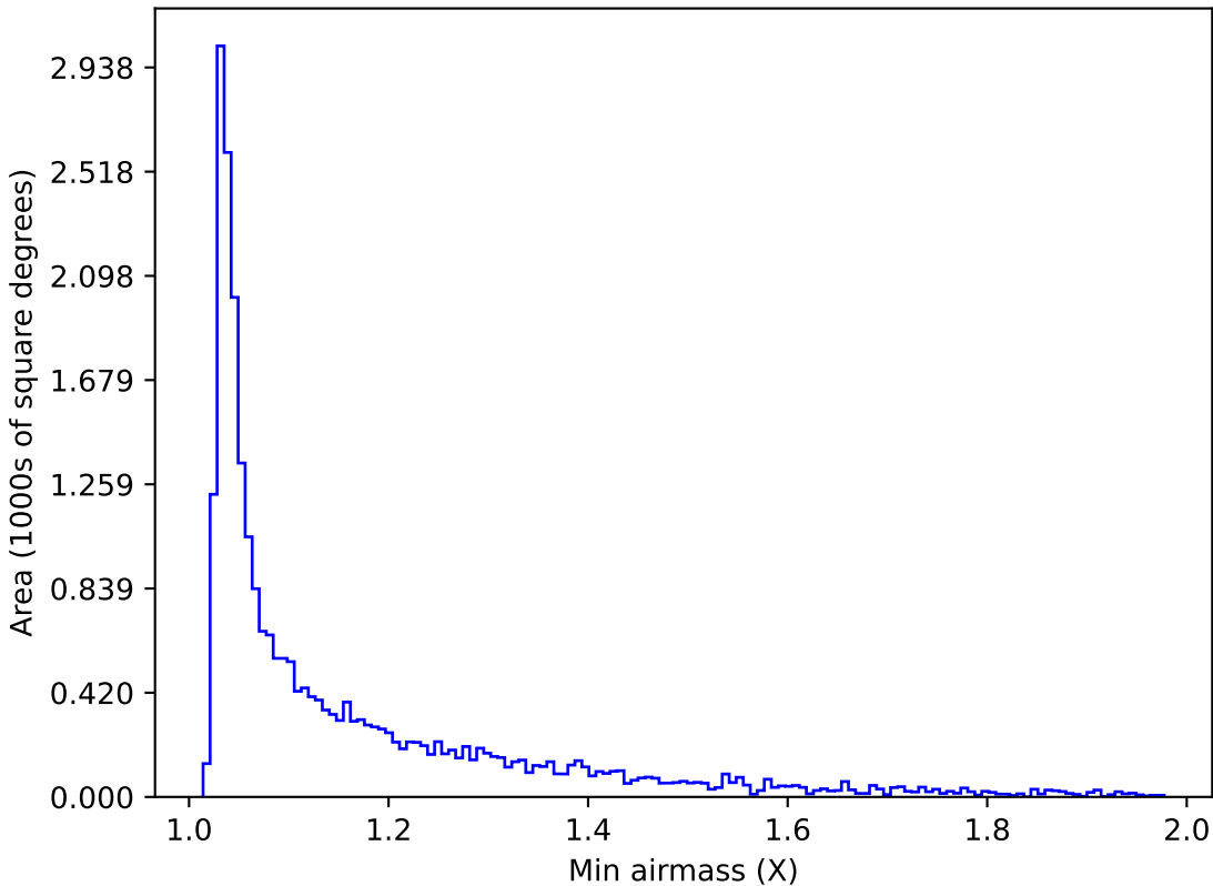
too_elab_heavy_r64_d3_griz_v3.4_10yrs Yr 1 i band: Min airmass
