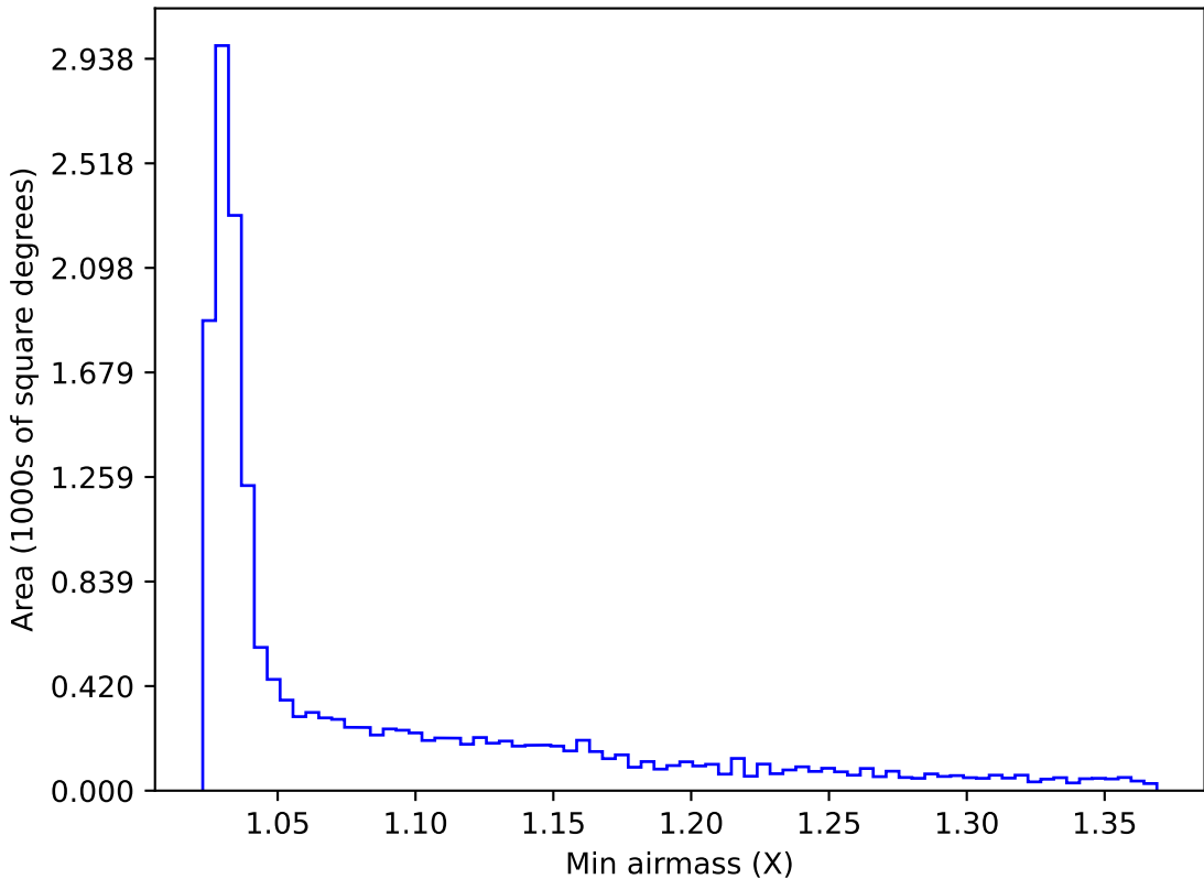
too_elab_heavy_r64_d3_griz_v3.4_10yrs WFD y band: Min airmass
