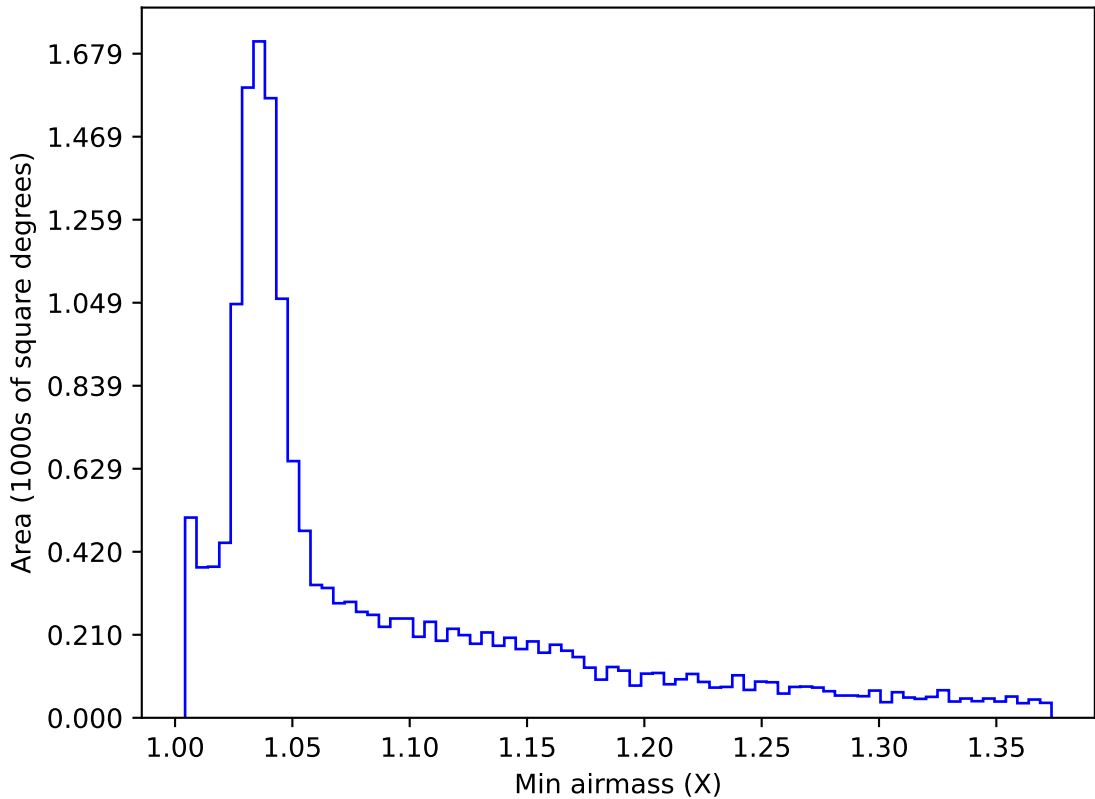
too_elab_heavy_r64_d3_griz_v3.4_10yrs WFD g band: Min airmass
