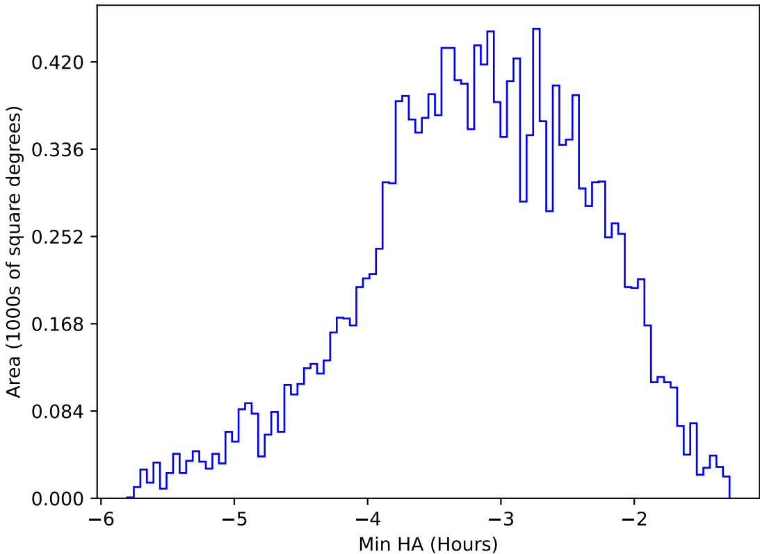
too_elab_heavy_r64_d3_griz_v3.4_10yrs WFD u band: Min HA
