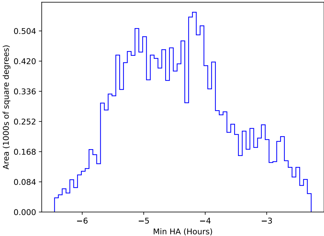
too_elab_heavy_r64_d3_griz_v3.4_10yrs WFD r band: Min HA
