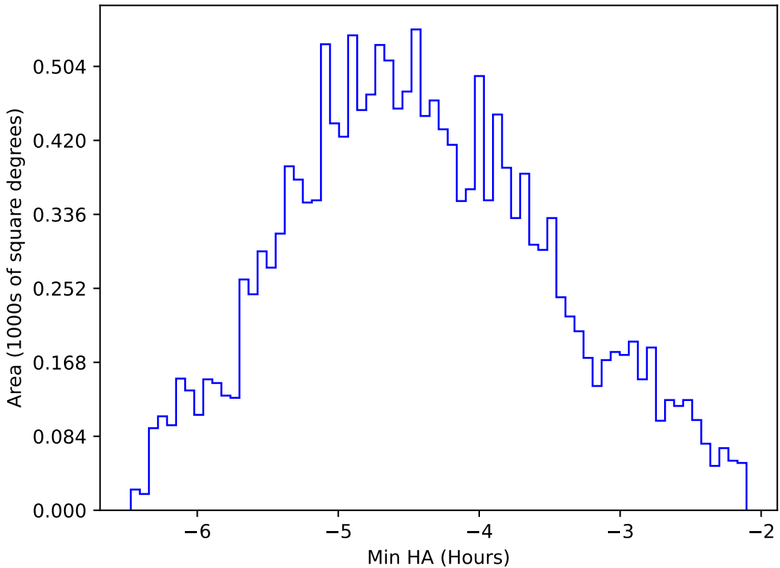
too_elab_heavy_r64_d3_griz_v3.4_10yrs WFD i band: Min HA
