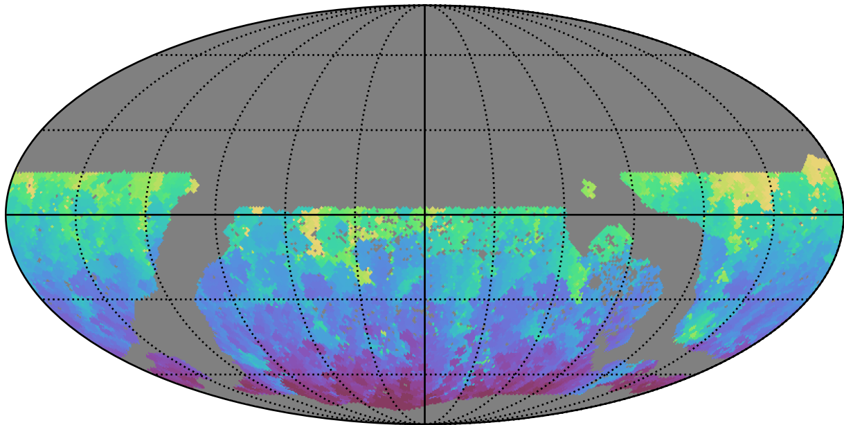
too_elab_heavy_r64_d3_griz_v3.4_10yrs WFD g band: Min HA
