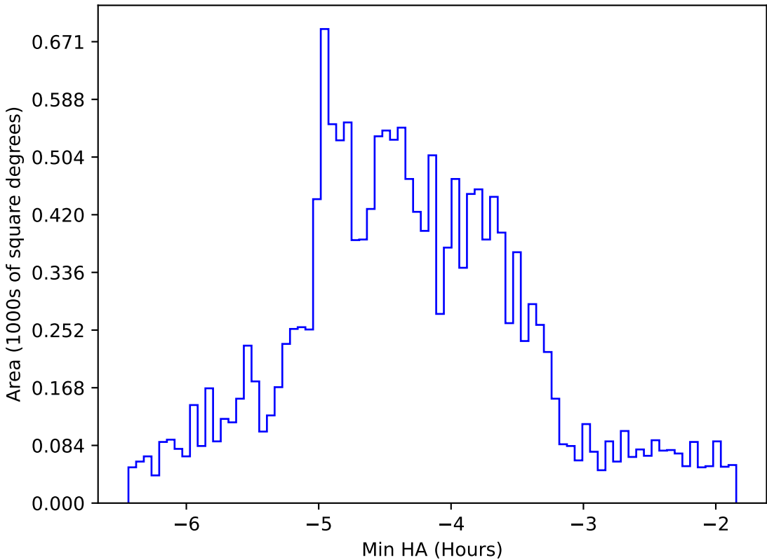
too_elab_heavy_r64_d3_griz_v3.4_10yrs WFD g band: Min HA
