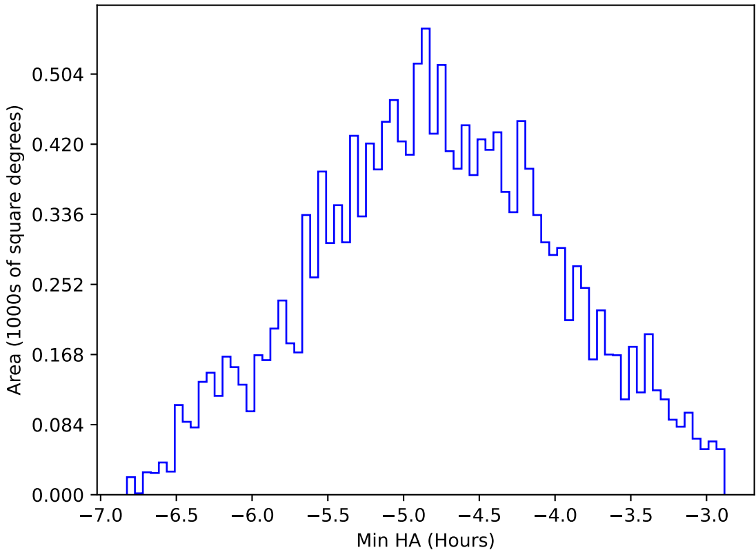
too_elab_heavy_r64_d3_griz_v3.4_10yrs WFD all bands: Min HA
